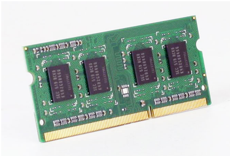
DIMM SO-DDR-3 2GB
